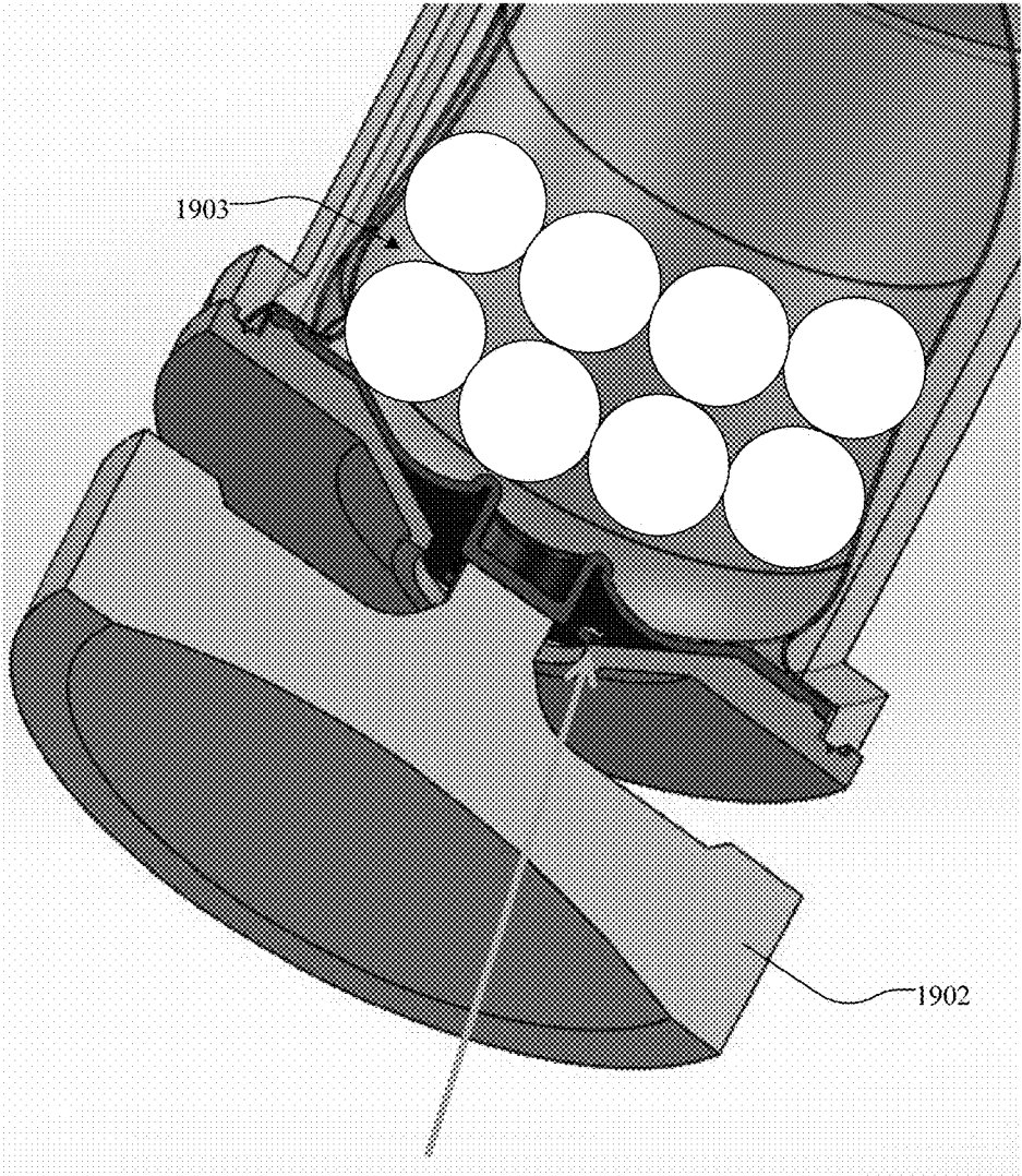
Breaking Mechanism for the Capsule(s)
